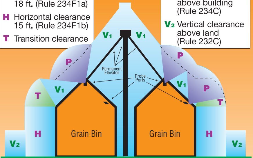
Clearance envelope for grain bins filled by permanently installed augers, conveyors or elevators
